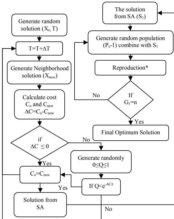
Fig. 2 Hybrid Simulated Annealing Genetic Algorithm (HSAGA)
