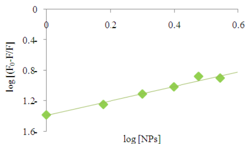
Fig. 5 Plot of \log [(F_0-F)/F] versus \log [NPs] to determine binding constant and the number of binding sites ( R^2=0.97 )
