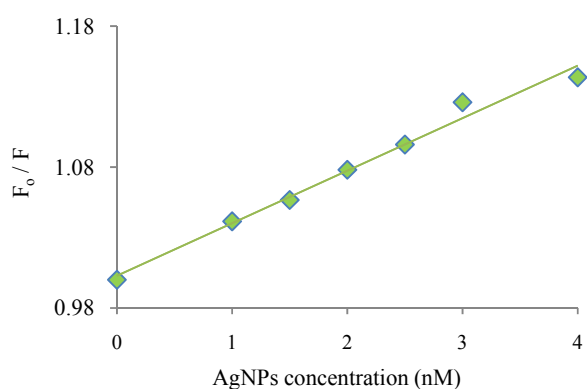
Fig. 3 Stern–Volmer plot. F_0/F = 0.0373 [NPs] + 1.0029 ( R^2=0.98 )
