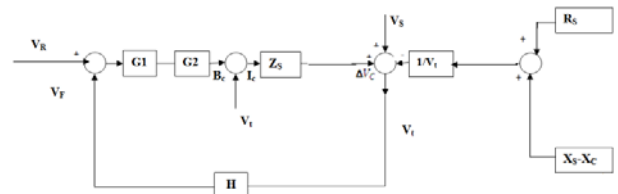
Fig. 4 Block diagram of a SVC and SC
