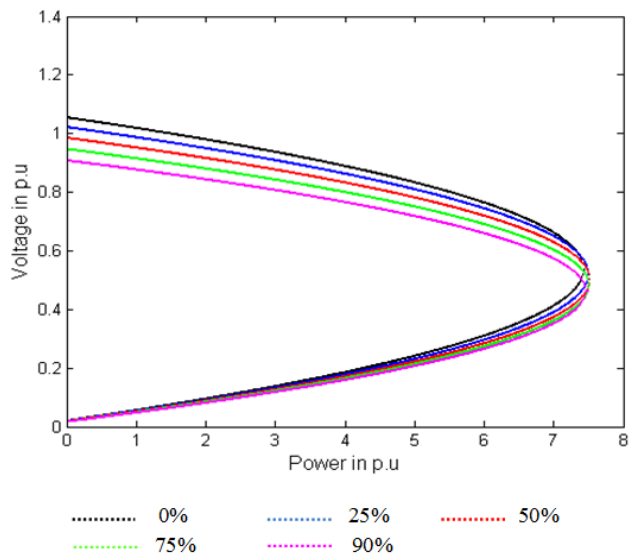
Fig. 6 P-V curve with different series compensation (0-90%), with constant Q and with G=0.0
