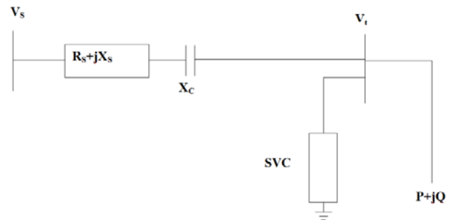
Fig. 3 Thevenin's equivalent system
