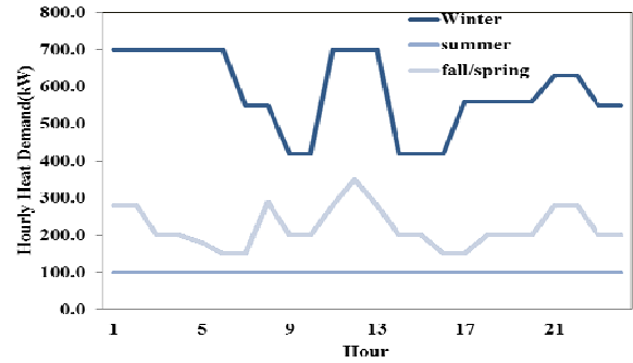
Fig. 4 Hourly heat demand for a typical hotel
