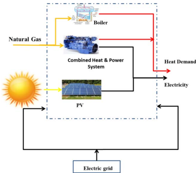
Fig. 2 Example of energy hub model for typical hotel
