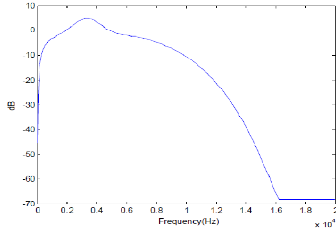
Fig. 3 The transfer functions of the external and middle ear model
