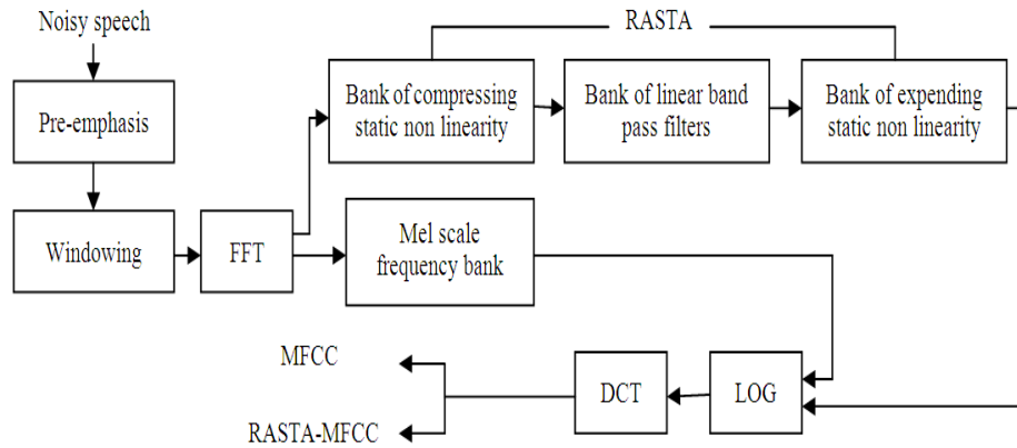
Fig. 1 Block diagram for extracting MFCC and RASTA-MFCC
