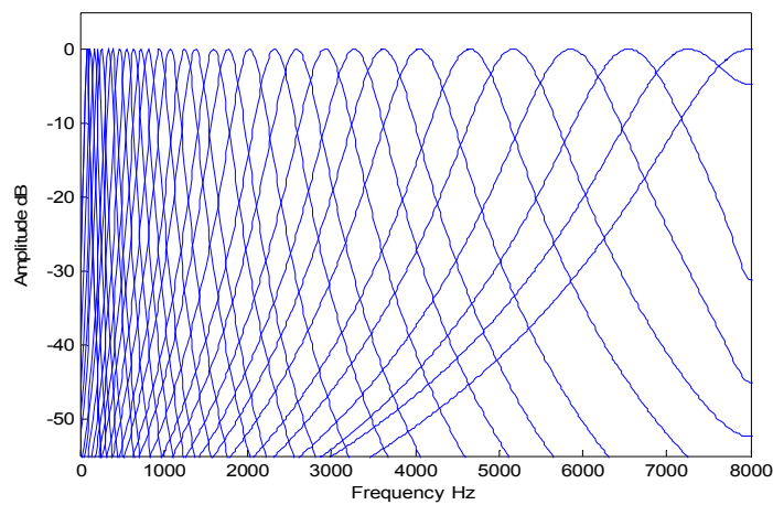
Fig. 4 Characteristics of gammachirp filterbank
