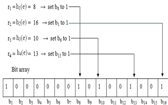
Fig. 1 Bloom Filter
