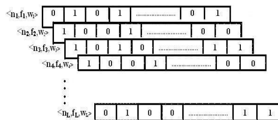
Fig. 2 Bin Bloom Filter
