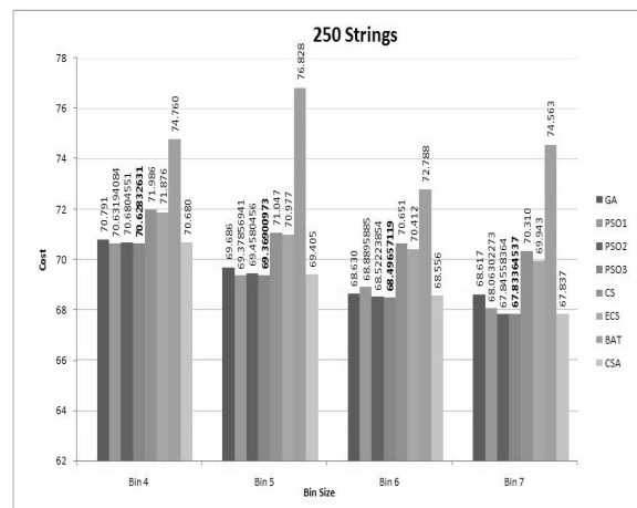
Fig. 4 Cost of BBF for synthetic dataset of 250 strings
