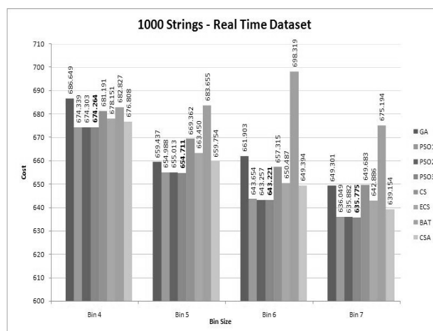
Fig. 7 Cost of BBF for real time dataset of 1000 strings
