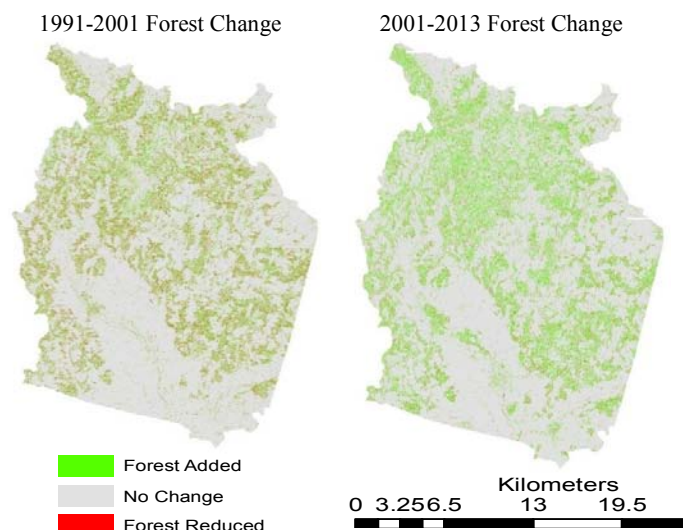
Fig. 3 Increase and decrease in forest cover
