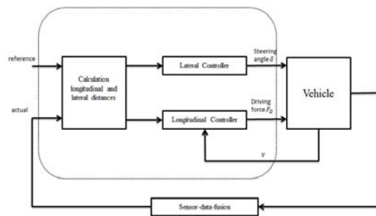
Fig. 4 Path controller
