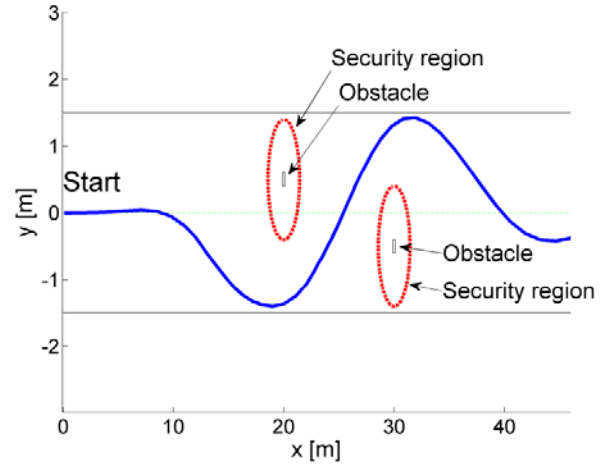
Fig. 9 Multi obstacle avoidance
