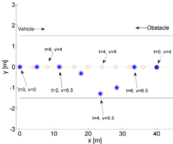
Fig. 11 Moving obstacle avoidance
