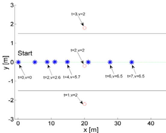
Fig. 12 Moving obstacle avoidance-Cyclist, pedestrian
