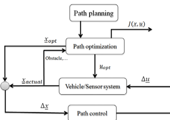
Fig. 1 General hierarchical concept of autonomous driving
