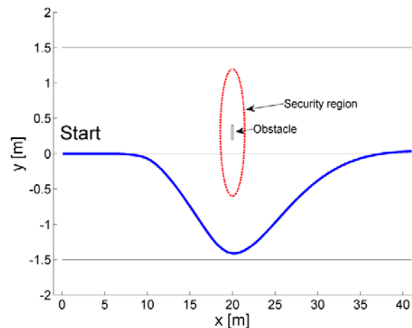
Fig. 6 Obstacle avoidance with elliptical security region
