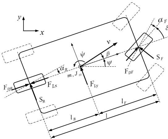
Fig. 2 Vehicle nonlinear single track model
