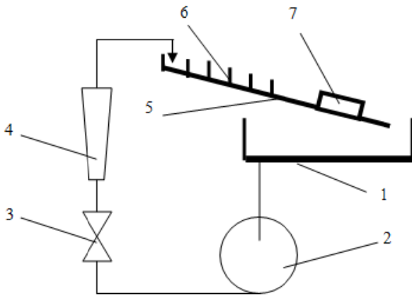
Fig. 1 Experimental setup
