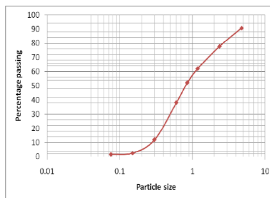
Fig. 1 Sand particle size distribution curve
