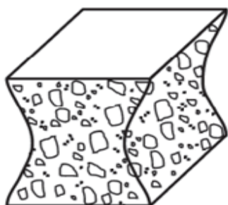
(b) Acceptable cube fracture shape
