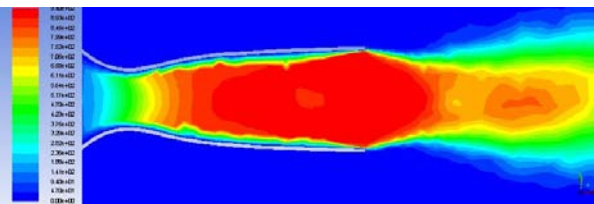
(e) Chevron with U-type edge
