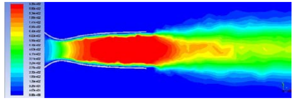
(c) Chevron with flat edge
