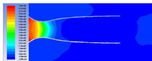
(a) Base model of the CD nozzle
