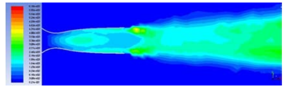
(c) Chevron with flat edge
