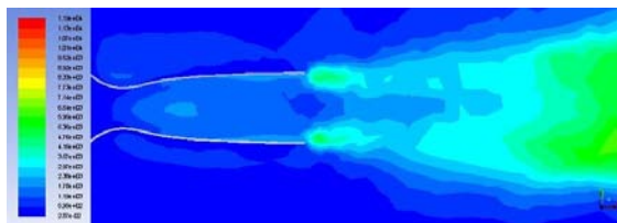
(a) Base model of the CD nozzle
