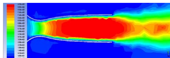
(a) Base model of the CD nozzle
