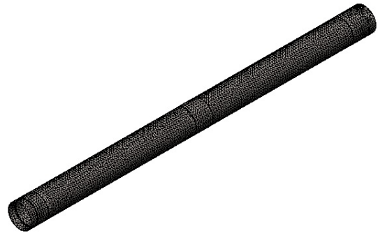
Fig. 8 Finite element grid of rocket motor case
