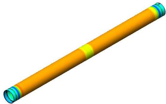
Fig. 9 Principal stress on rocket motor case
