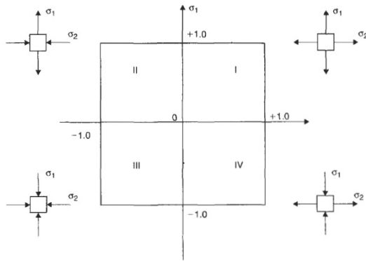
Fig. 2 Graph of maximum principal stress theory
