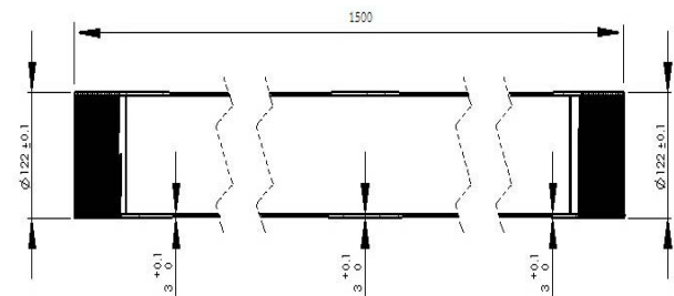
Fig. 4 Rocket motor case geometry
