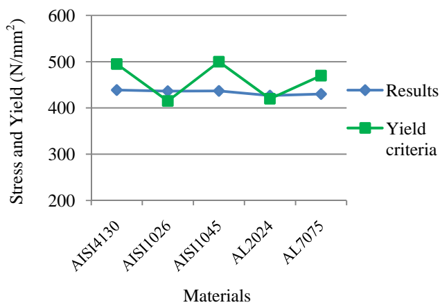
Fig. 11 The principal stress with yield criteria
