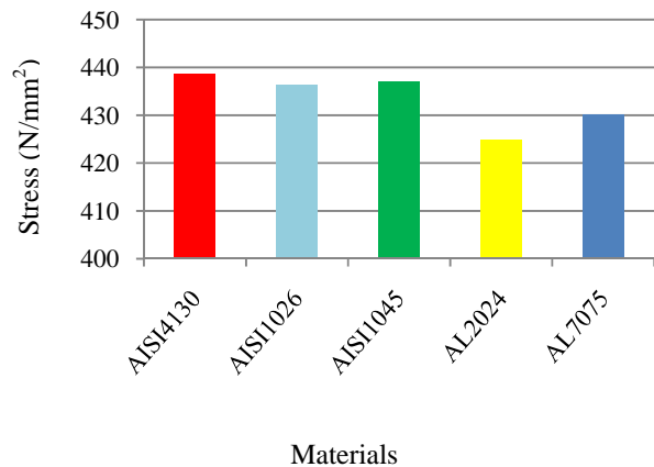
Fig. 10 The principal stress on material surface
