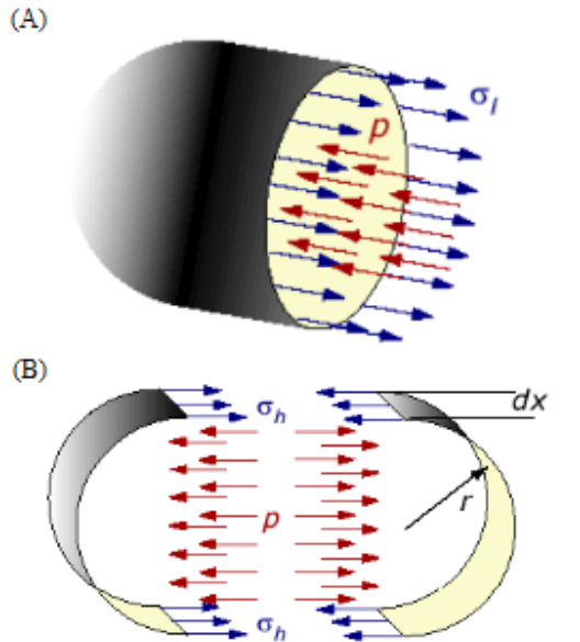
Fig. 1 Stress direction on thin-wall pressure vessel (A) longitudinal stress and (B) circumferential stress on material surface
