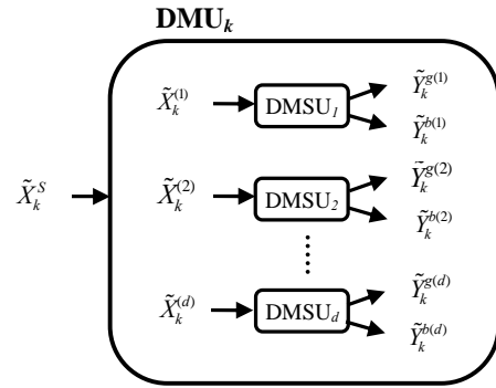
Fig. 2 Multi-component DMU_k in fuzzy DEA
