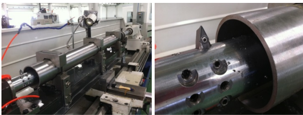
Fig. 1 (a) Workpiece and machine setup for modified boring tool on lathe machine, (b) V-shaped carbide cutting insert equipped on a spinning mandrel
