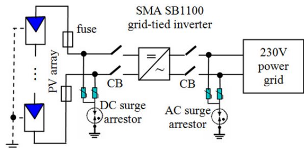
Fig. 3 The structure of PV systems
