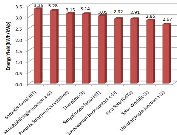
Fig. 6 Energy yields of 9 PV systems
