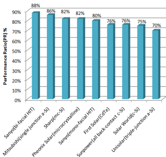
Fig. 7 Performance ratios (PR) of 9 PV systems
