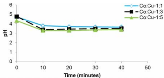
Fig. 4 pH for synthetic solutions with 25g 0.02M HCl activated clinoptilolite
