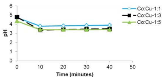
Fig. 3 pH for synthetic solutions with 15 g 0.02M HCl activated clinoptilolite
