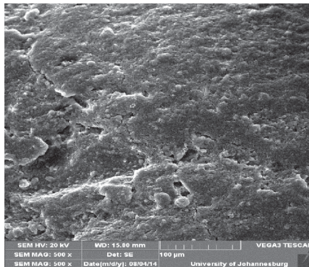
Fig. 2 SEM of 0.02HCl activated clinoptilolite
