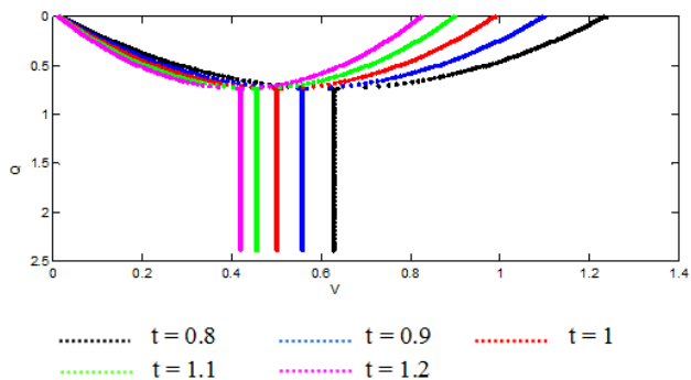
Fig. 9 VQ curve with different off-nominal tap ratios (0.8-1.2).
