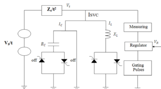
Fig. 5 SVC and power system schematic
