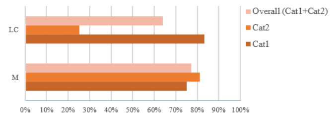
Fig. 4 Impact of M and LC on classes with poor R
