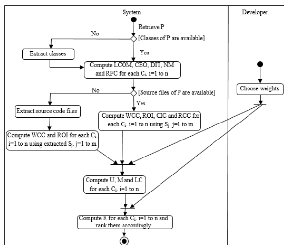
Fig. 1 Reusability Assessment Approach
