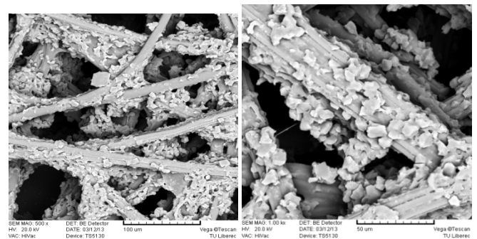
Fig. 4 Scanning electron microscope images of aerogel treated nonwoven fabrics
