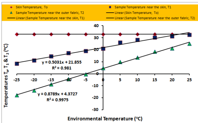
Fig. 7 Temperature gradient graph for Sample 2
