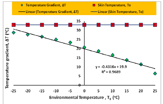
Fig. 10 Temperature gradient graph for Sample 3
