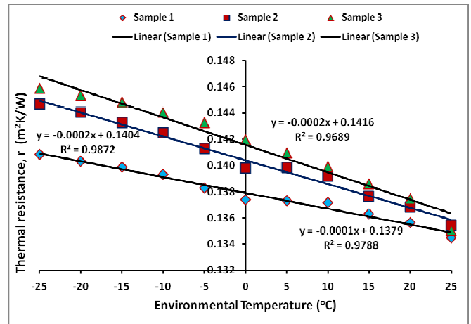
Fig. 12 Thermal resistance Vs Environmental temperature
