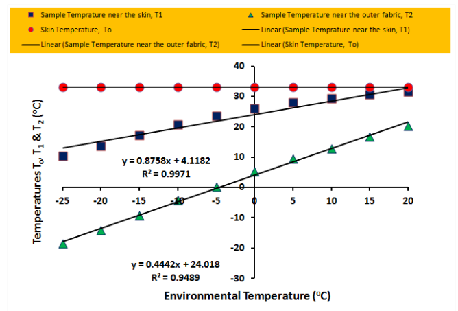
Fig. 9 Temperature variation graph for Sample 3
