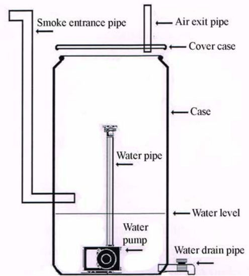
Fig. 3 A smoke and smell filter case design
