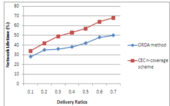
Fig. 9 Delivery Ratios vs. Network Lifetime
