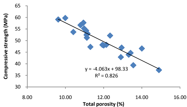
Fig. 9 Relationship between compressive strength and total porosity
