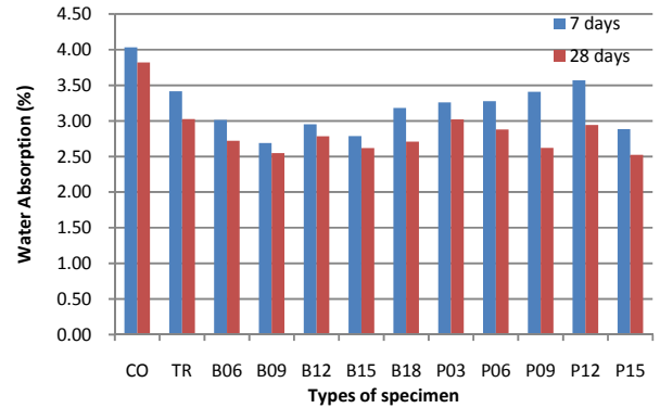
Fig. 7 Water absorption of all specimens at different curing ages
