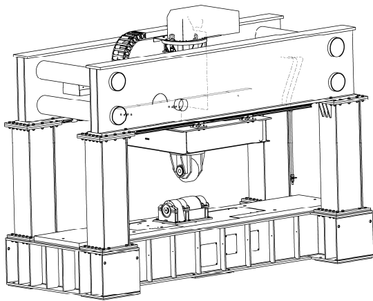
Fig. 3 Machine MGPS-100, capacity 1000 kN (100 t)
