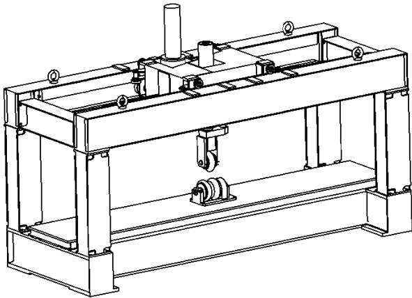
Fig. 2 Machine MGPS-25, capacity 250 kN (25 t)
