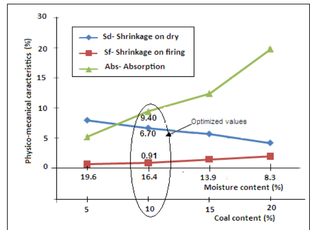
Fig. 5 Shrinkage variation and absorption in relation with moisture of mixtures according the particle size (1.60 mm) and coal content
