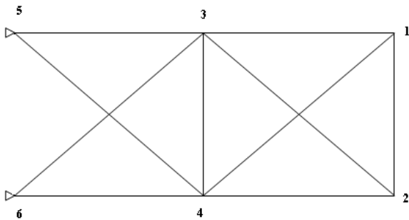
Fig. 1 Structure of 10- bar plane truss
