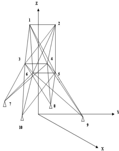
Fig. 2 Structure of 25- bar space truss
