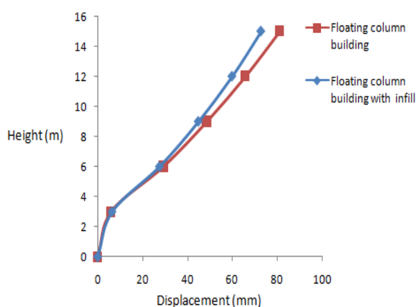
Fig. 3 Lateral floor displacement
