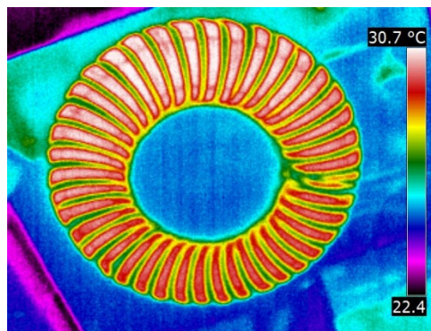
Fig. 9 Thermal image of axial fluke Komel's generator winding
