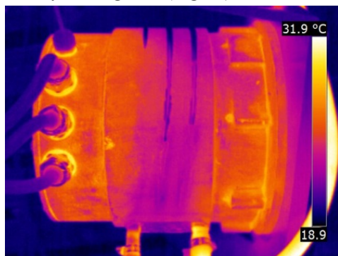
Fig. 11 Thermal image cooling duct of motor of type SMwsPA132S4
