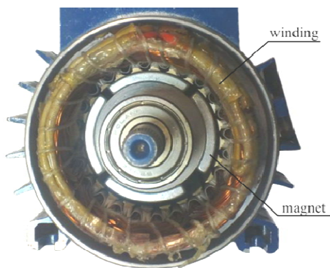
Fig. 14 Permanent machine
