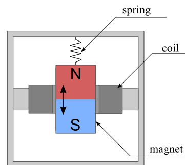
Fig. 13 The electrodynamic sensor
