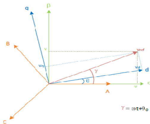
Fig. 6 3-phase Voltage transformations
