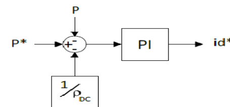
Fig. 10 Power Control
