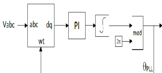
Fig. 8 Phase Lock Loop Scheme
