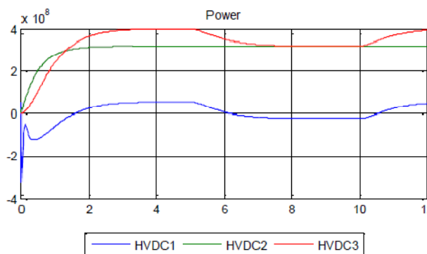
Fig. 13 (c) 3 Terminal MTDC with changed Voltage and Power References
