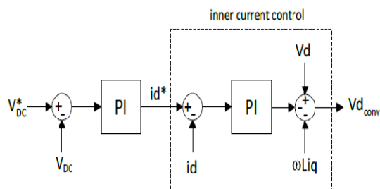
Fig. 9 Voltage Control Scheme
