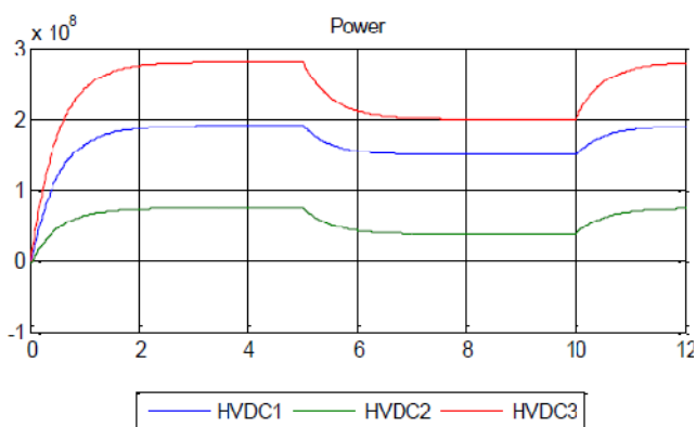
Fig. 14 (c) Voltage and Power with Droop Control
