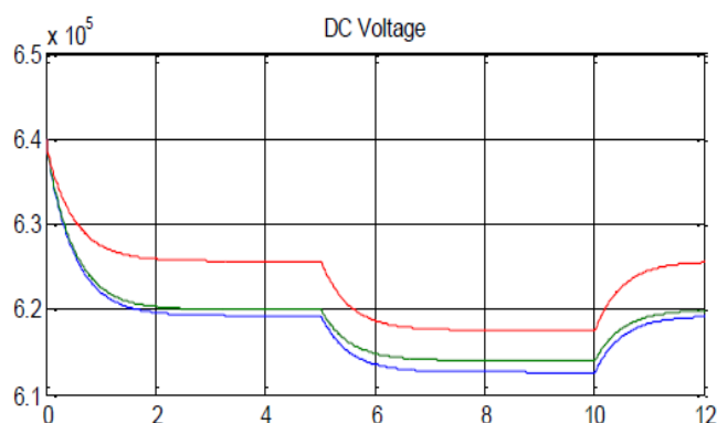
Fig. 14 (b) Voltage and Power with Droop Control
