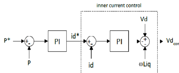
Fig. 10 Power Control
