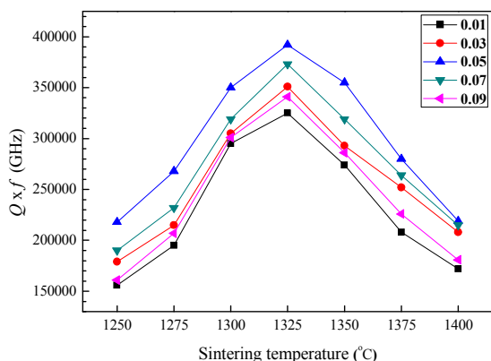
Fig. 6 Q \times f values of (Mg_{1-x}Ni_x)_2(Ti_{0.95}Sn_{0.05})_2O_4 ( x=0.01 \sim 0.09 ) ceramics system sintered at different temperatures
