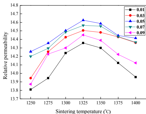
Fig. 5 Relative permittivity of (Mg_{1-x}Ni_x)_2(Ti_{0.95}Sn_{0.05})_2O_4 ( x=0.01-0.09 ) ceramics sintered at different temperatures
