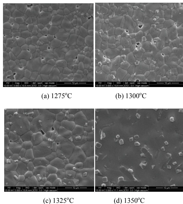
Fig. 3 SEM photographs of (Mg_{0.95}Ni_{0.05})_2(Ti_{0.95}Sn_{0.05})O_4 ceramics sintered at (a) 1275, (b) 1300, (c) 1325 (d) 1350 °C, respectively
