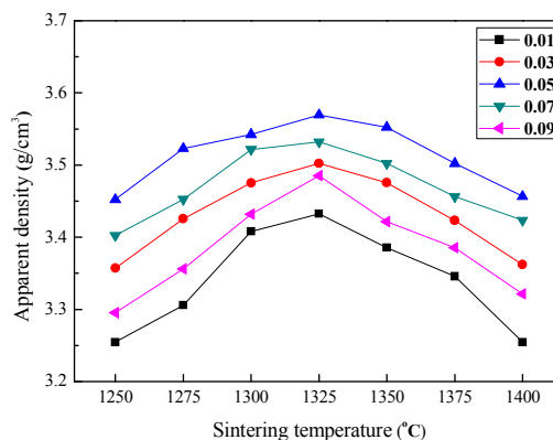
Fig. 4 Apparent densities of (Mg_{1-x}Ni_x)_2(Ti_{0.95}Sn_{0.05})O_4 ( x = 0.01 - 0.09 ) ceramics sintered at various sintering temperatures
