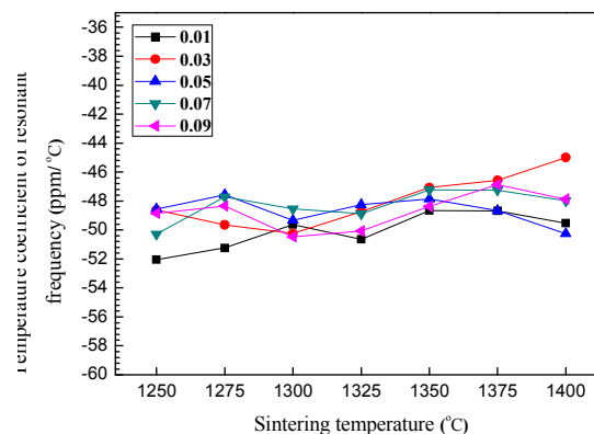
Fig. 7 Temperature coefficient of resonant frequency values of (Mg_{1-x}Ni_x)_2(Ti_{0.95}Sn_{0.05})_2O_4 ( x=0.01 \sim 0.09 ) ceramics sintered at different temperatures
