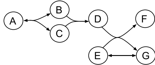
(b) Directed hypergraph
