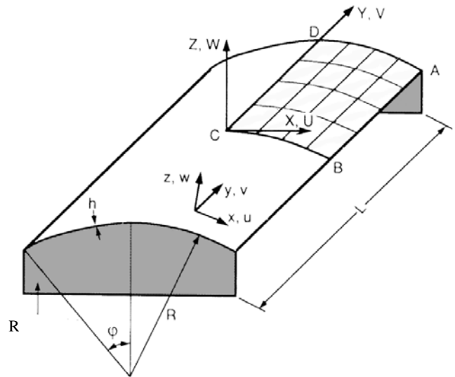
Fig. 8 Scordelis-Lo roof
