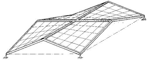
Fig. 3 Gable roof hyperbolic paraboloid shell
