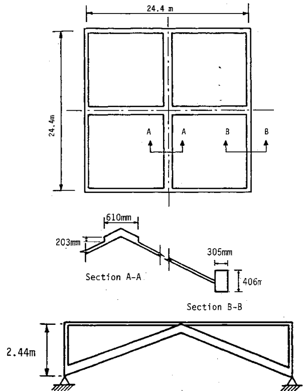
Fig. 4 Gable roof dimensions and configuration
