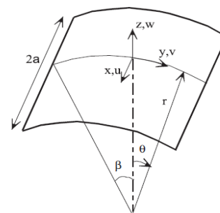
Fig. 1 Shell element
