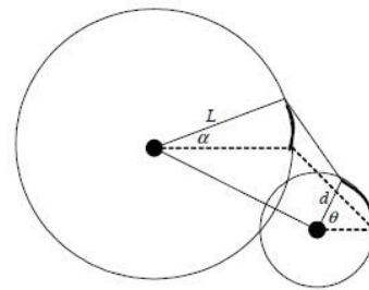
Fig. 3. Relation between motor position and beam angle
