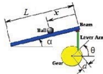
Fig. 2. Schematic diagram
