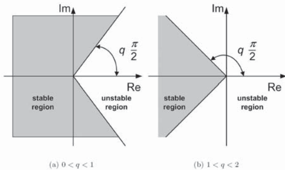
Fig. 5. Stability region of LTI fractional order systems
