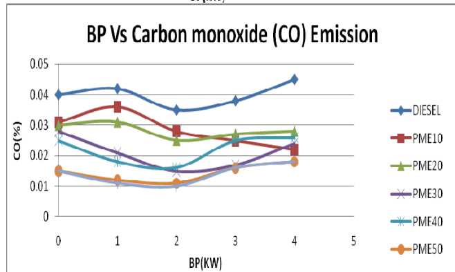
Fig. 8 Variation of carbon monoxide for PME, its Blends and diesel for CR 17.5 and 18.5
