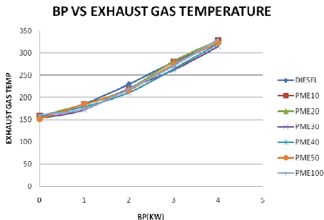
BP VS EXHAUST GAS TEMPERATURE
