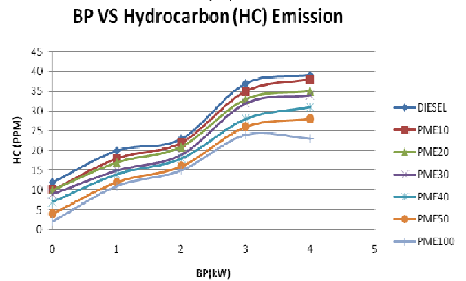
Fig. 9 Variation of Hydrocarbons for PME, its blends and diesel for CR 17.5 and 18.5
