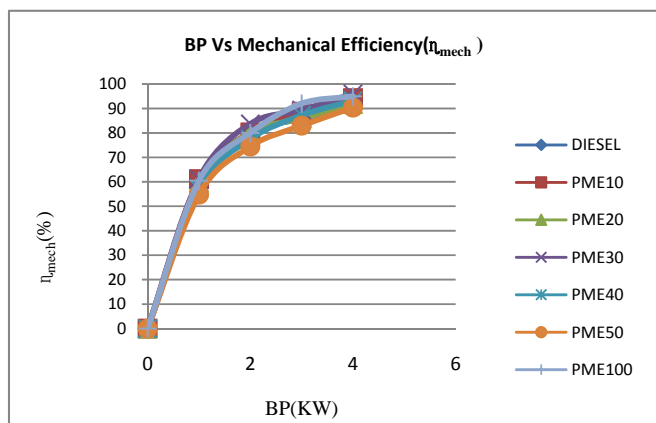
BP Vs Mechanical efficiency
