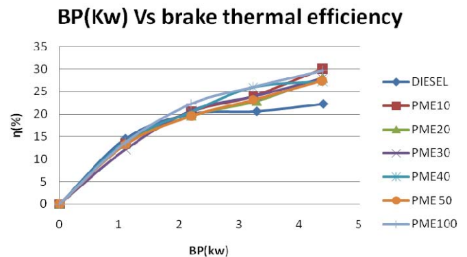
Fig. 2 Variation of brake thermal efficiency for PME, its Blends and diesel at CR 17.5 and 18.5
