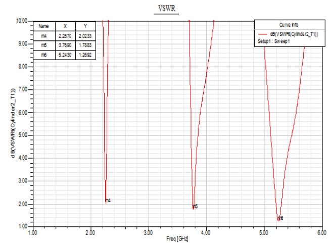
Fig. 3 (b) VSWR of proposed antenna
