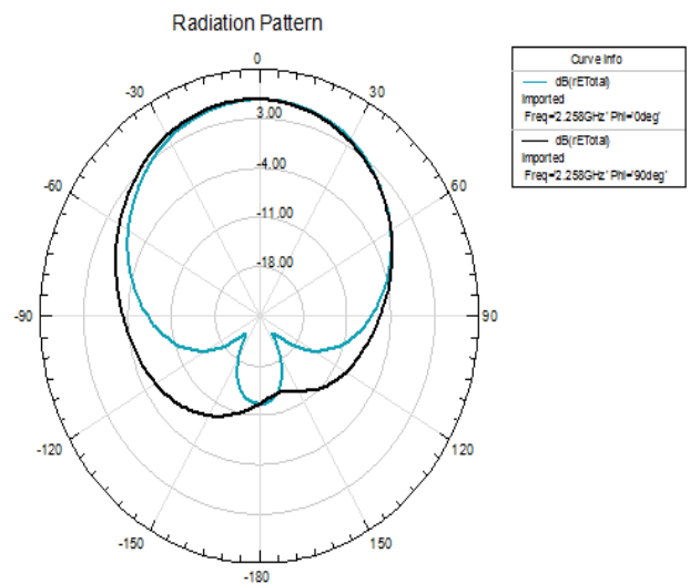
Fig. 3 (c) Simulated radiation pattern at 2.256 GHz
