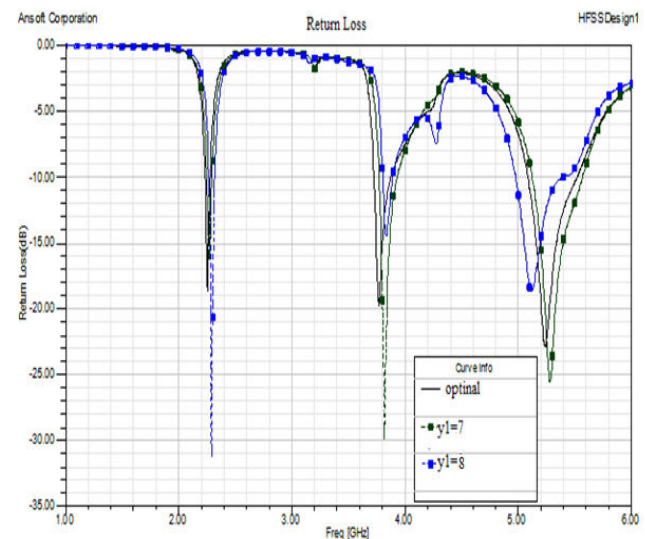
Fig. 5 Simulated return loss for different values of 'y1'
