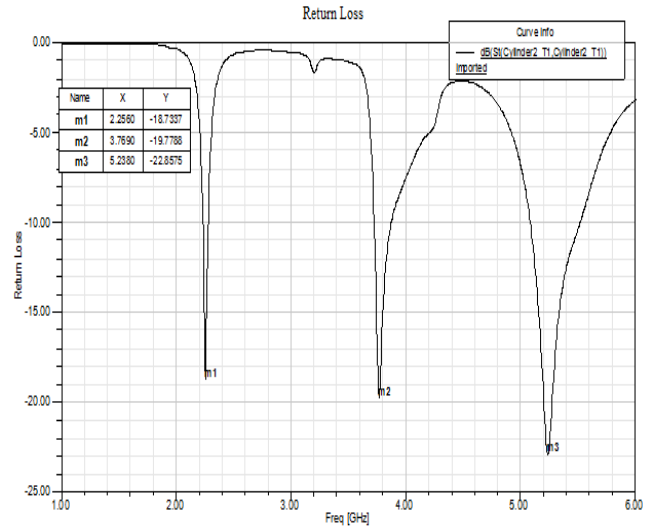
Fig. 3 (a) Simulated return loss for proposed antenna
