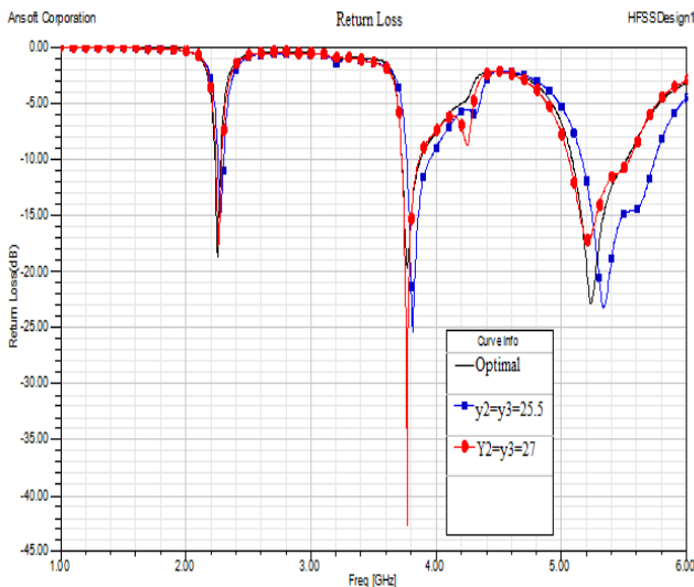
Fig. 7 Simulated return loss for different values of 'y2' & 'y3'
