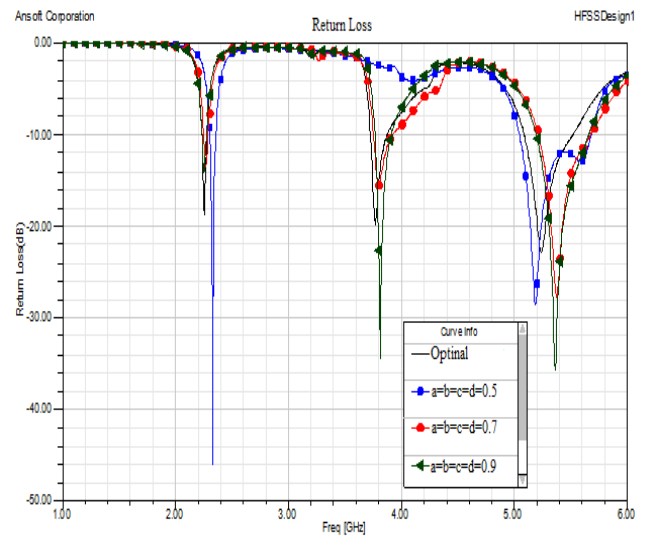
Fig. 4 Simulated return loss for different values of 'a', 'b', 'c', 'd'
