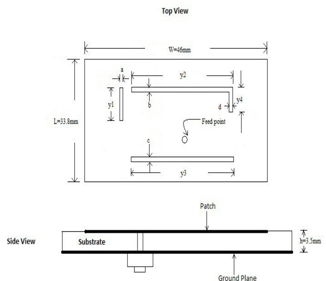
Fig. 1 Schematic diagram of proposed antenna
