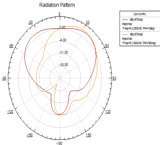
Fig. 3 (e) Simulated radiation pattern at 5.238 GHz
