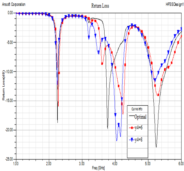
Fig. 6 Simulated return loss for different values of 'y4'
