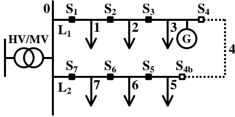
Fig. 6 Example of reconfigurable network
