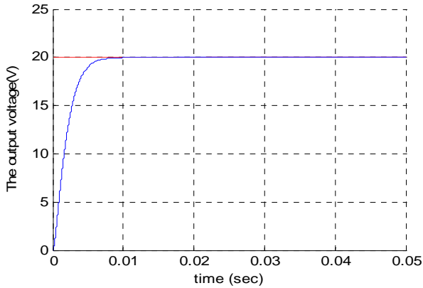
(f) Output voltage for load variation
