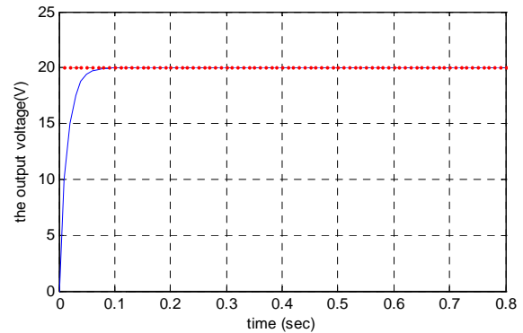
(a) Output voltage for a 20v reference
