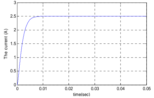
(b) Inductor current for a 20 v reference
