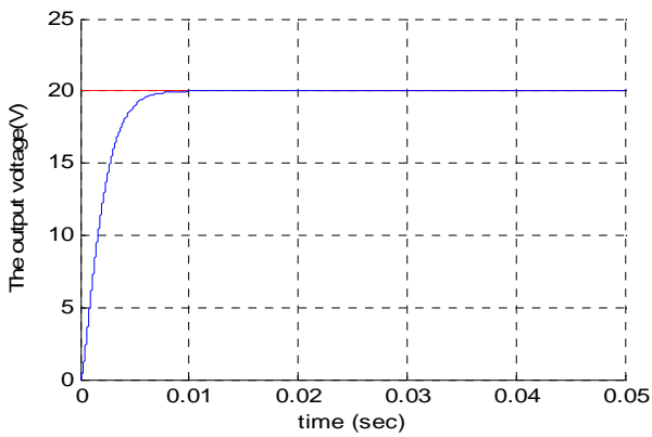
(a) Output voltage for a 20v reference
