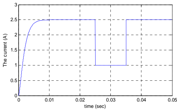
(g) Inductor current for load variation
