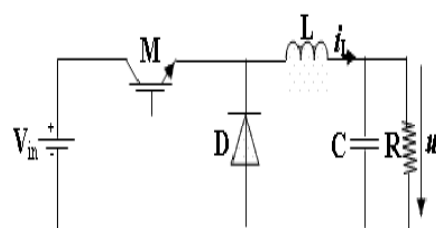
Fig. 1 DC-DC Buck converter
