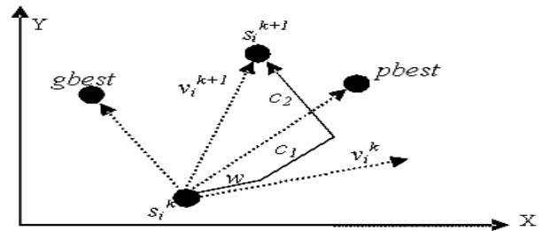
Fig. 2 The velocity and position updates in PSO
