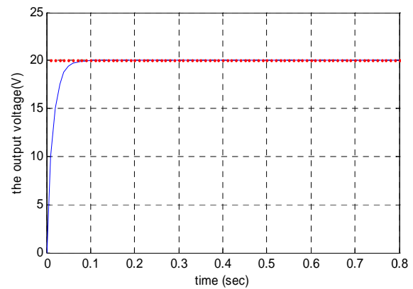
(c) Output voltage for line variation
