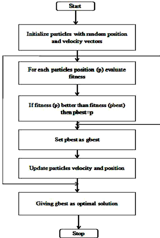
Fig. 3 PSO algorithm
