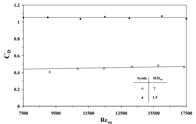
Fig. 6 Drag coefficient of cam-shaped tube
