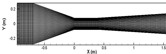
Fig. 1 Computational Grid
