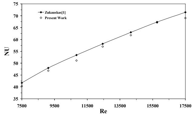
Fig. 5 Heat transfer circular tube in cross-flow
