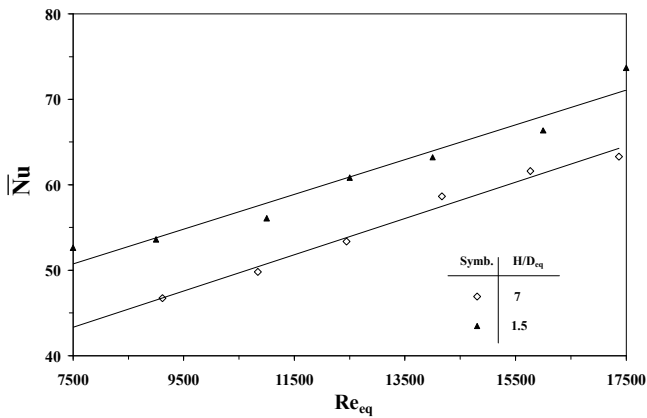
Fig. 7 Heat transfer from cam-shaped tube
