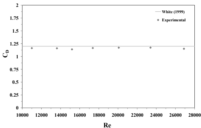
Fig. 4 Drag coefficient of circular tube in cross-flow
