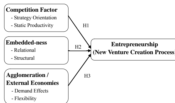
Fig. 1 Research Model
