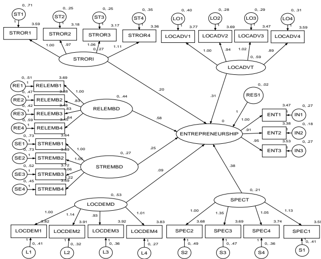
Fig. 3 AMOS Model
