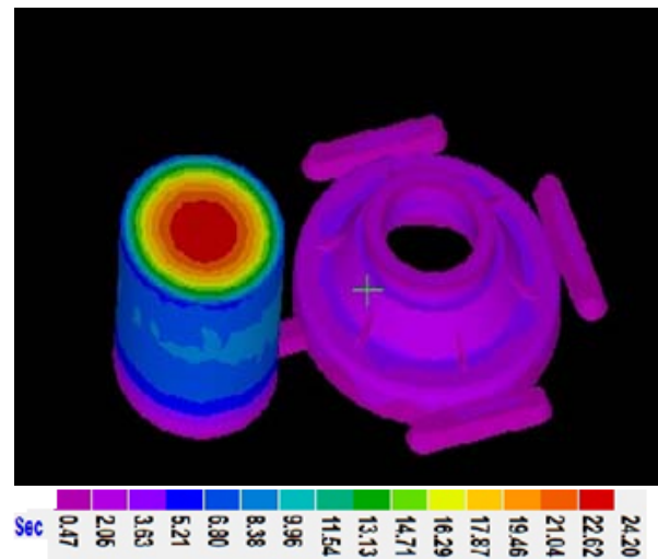
Fig. 6 Contour of solidification time
