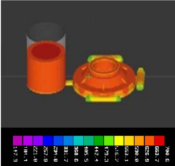
Fig. 7 Contour of temperature distribution 7.31 seconds after injection
