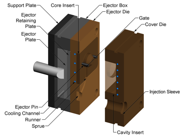
Fig. 1 Die assembly and components (cold chamber) [1]
