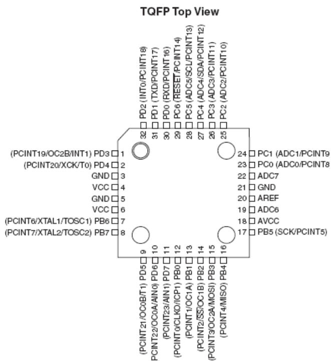
Fig. 3 ATmega48/88/168 Microcontroller
