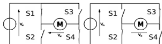
Fig. 6 The two basic states of an H-bridge
