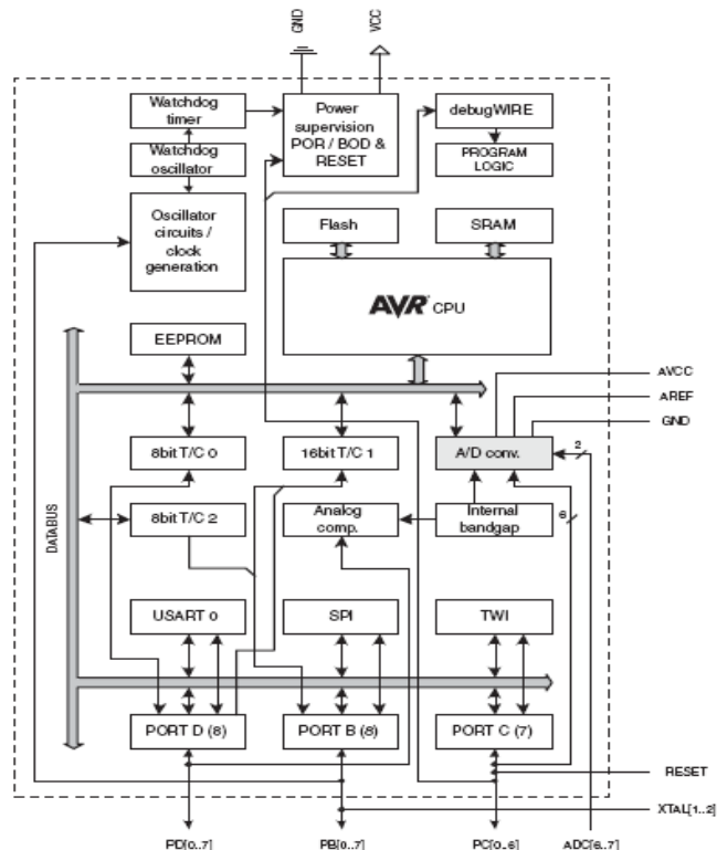
Fig. 4 Block diagram of the ATmega48/88/168 Microcontroller
