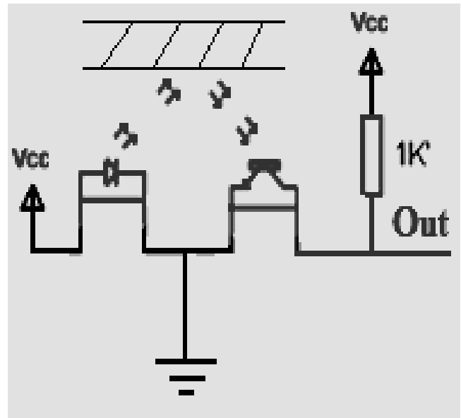
Fig. 11 Object detector electric circuit
