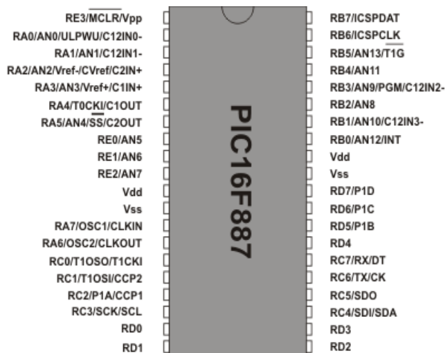
Fig. 1 PIC16F887 PDIP 40 Microcontroller
