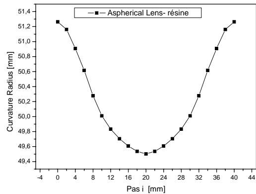
Fig. 5 Radius of curvature R i according to step of measurement i of the aspheric lens
