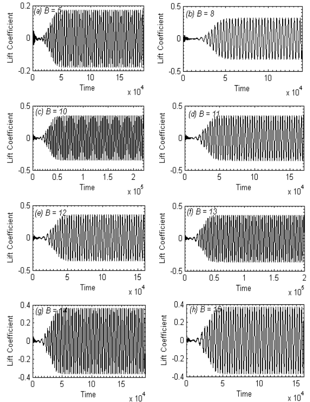
Fig. 15 Lift coefficient time-trace analysis at Re = 150 for various blockages
