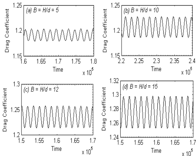
Fig. 14 Drag coefficient time-trace analysis at Re = 150 for various blockages
