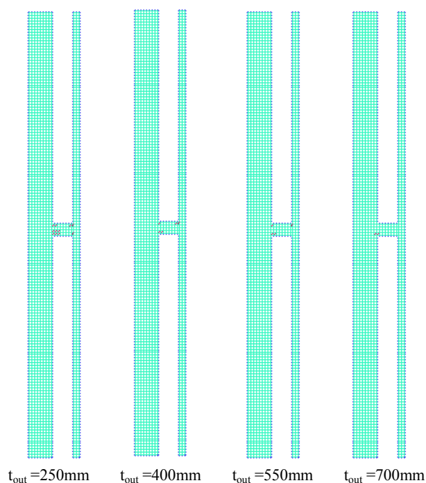
Fig. 5 Crack patterns for different outrigger thickness at 5 sec
