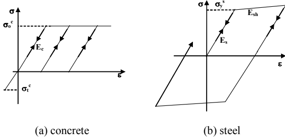
Fig. 1 Uni-axial stress- strain curves for cyclic loading [1]
