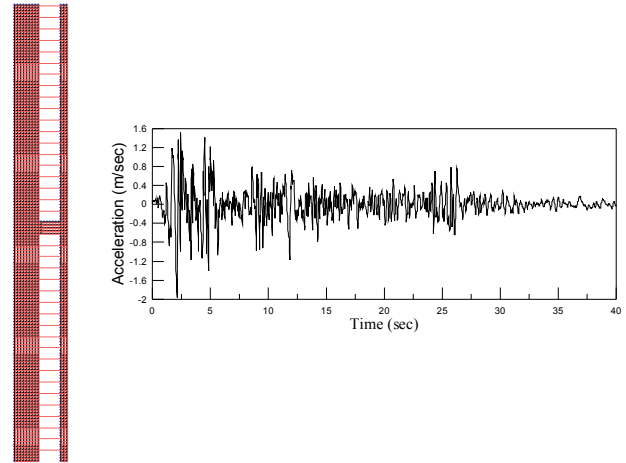
Fig. 2 Finite element model and earthquake records; El-Centro, 1940
