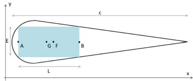
Fig. 5. Rectangular cross section within the airfoil
