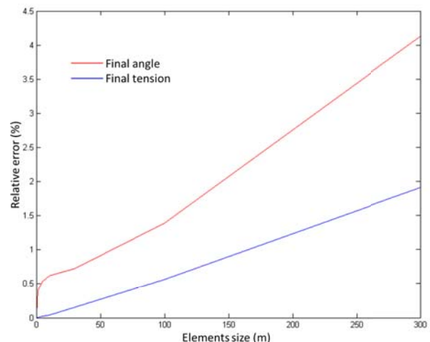
Fig. 19. Relative error vs. elements size
