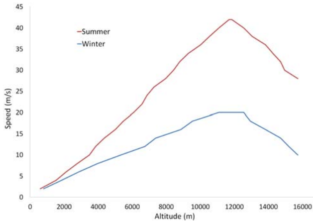
Fig. 10. Wind profile as a function of altitude
