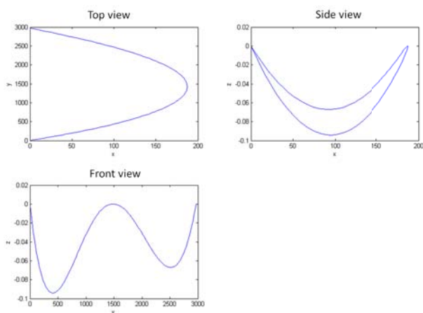
Fig. 23. Cable after a double rotation
