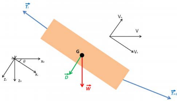
Fig. 11. Equilibrium of a small piece of the discretized cable
