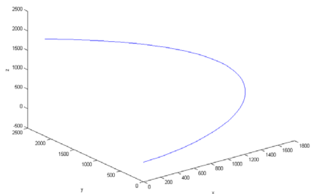
Fig. 22. 3D-visualization of the shape of the cable
