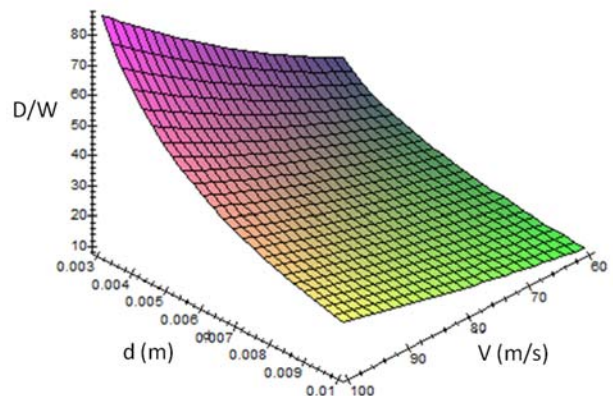
Fig. 15. Ratio drag over weight with respect to the effective speed and the diameter of the cable
