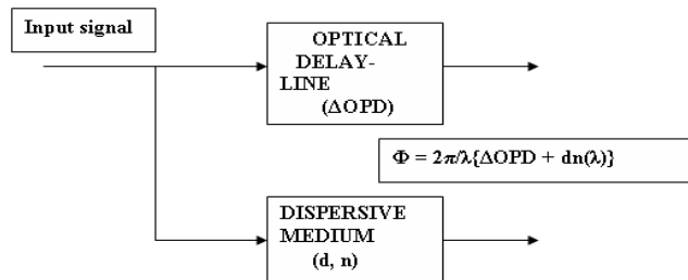
Fig. 5 Dispersion type phase-shifter
