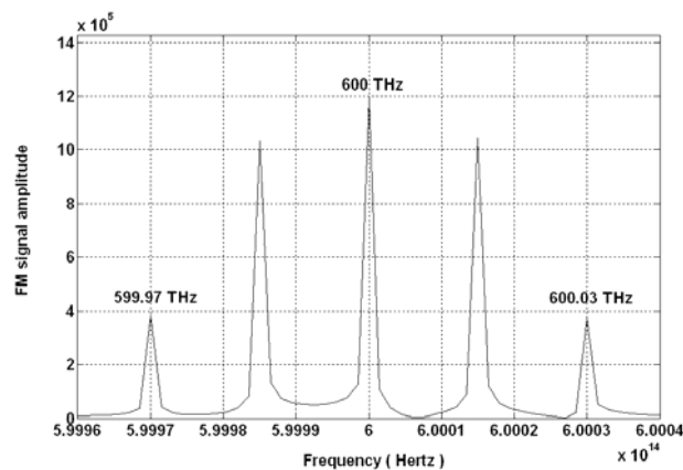
Fig. 2 FM spectrum of modulated master laser
