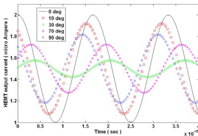
Fig. 6 Effect of phase de-coherence between the two slave laser sources
