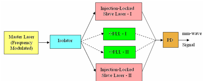
Fig. 1 The scheme for generation of ultra-stable millimeter-wave signal
