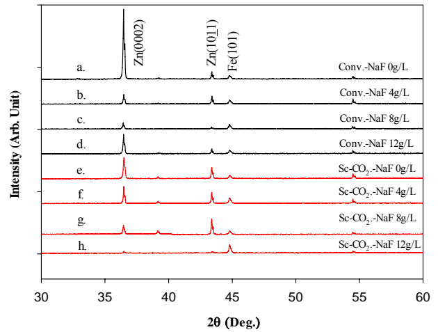
Fig. 7 The X-ray diffraction spectra for coatings prepared from both conventional and supercritical processes, respectively, and with different NaF concentrations.
