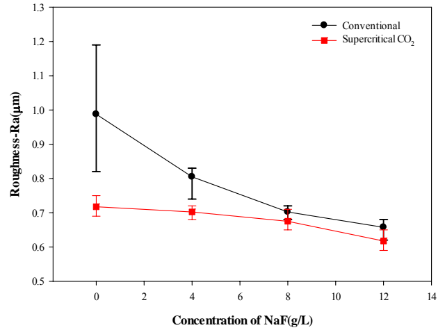
Fig. 6 The measured surface roughness of coatings prepared from electrolytes with different NaF concentrations
