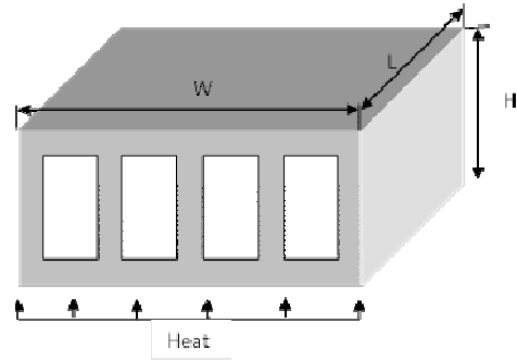
Fig. 1 Micro-channel heat sink
