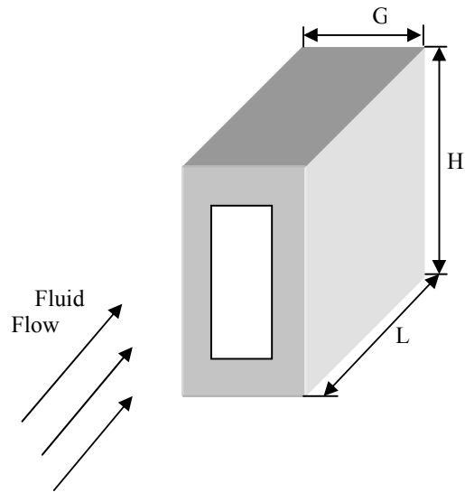
Fig. 2 Computational domain of micro channel heat sink
