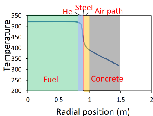
Fig. 7 Radial temperature distribution of normal storage
