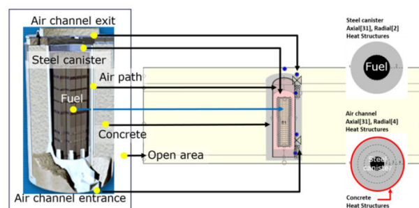
Fig. 2 TRACE model of Kuosheng NPP dry-storage system
