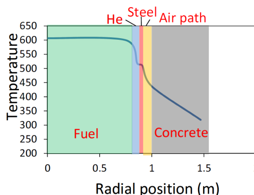
Fig. 10 Radial temperature of fully-blockage
