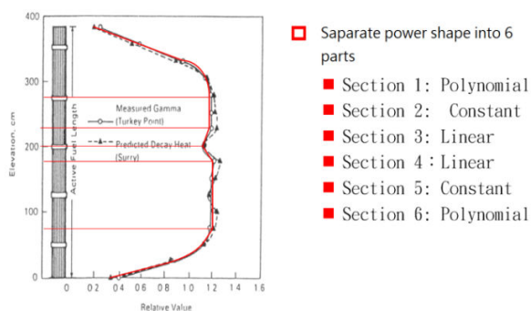
Fig. 4 Power distribution of VSC-17
