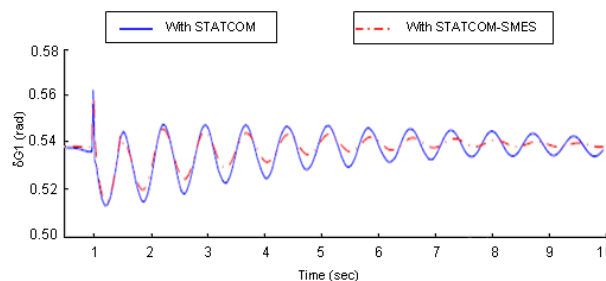
Fig. 8 Variation of rotor power angle
