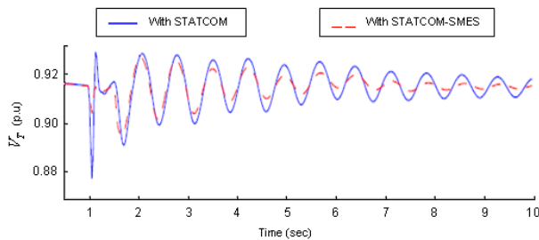
Fig. 10 Variation of compensator terminal voltage
