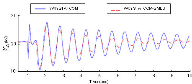
Fig. 11 Variation of compensator dc bus voltage
