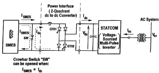
Fig. 1 General model of a STATCOM/SMES compensator
