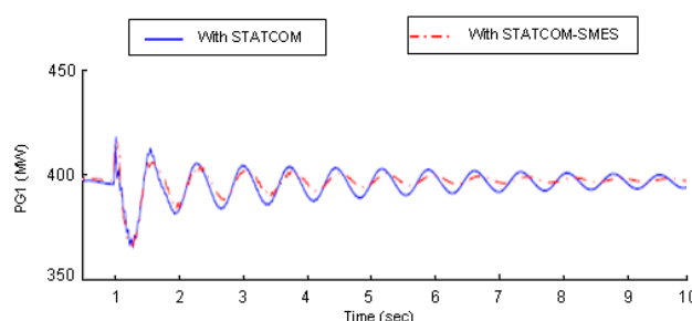
Fig. 7 Variation of generator active power
