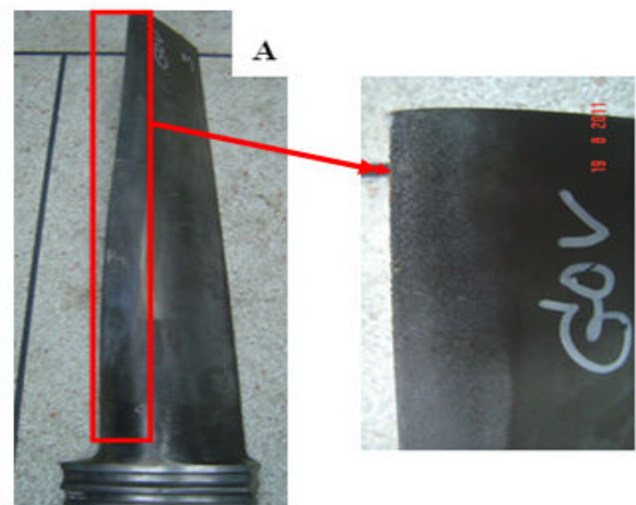
Fig. 1 Steam turbine blade showing damage caused by wear along the edge of the blade
