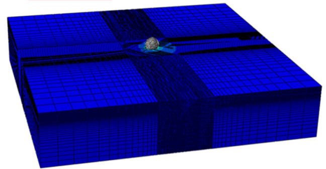
Fig. 3 FE collision model showing particle and surface
