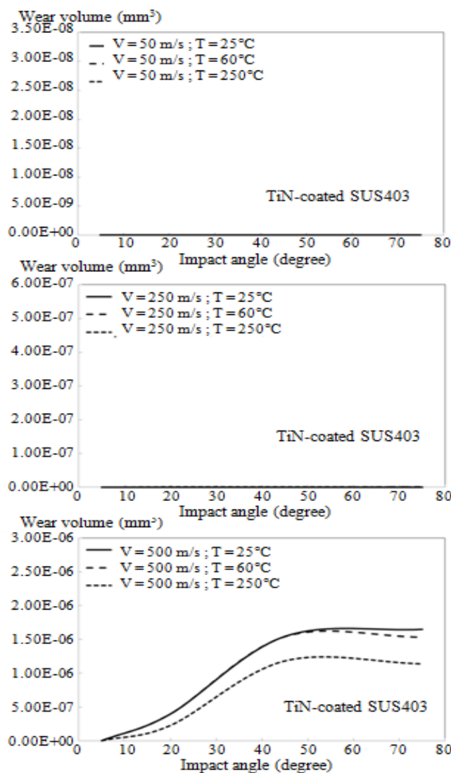
Fig. 6 The wear volume at different impingement angles, impingement speed and temperature for TiN-coated SUS403
