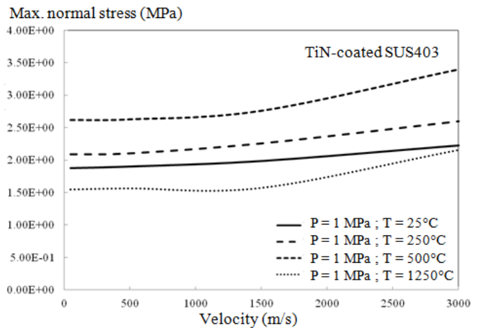
Fig. 11 Normal stress on TiN-coated SUS403 due to fluid jet of pressure 1 MPa at different velocity and temperature
