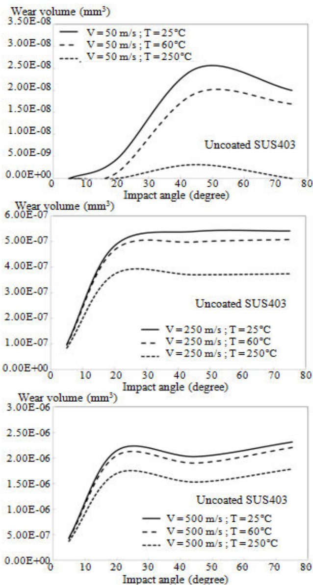
Fig. 5 The wear volume at different impingement angles, impingement speed and temperature for uncoated SUS403
